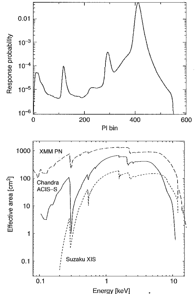
Fig. 4.11 [Top] One row of the ACIS-I response matrix showing the probability of a 6 keV input X-ray falling in each PI bin. [Bottom] Effective area curves for the three X-ray missions: XMM-Newton EPIC-pn detector (dashed line), Chandra ACIS-S (solid line), and Suzaku XIS-BI (dotted line). The effective-area curves were obtained from PIMMS 4.1 at http://heasarc.gsfc.nasa.gov/Tools/w3pimms.html
