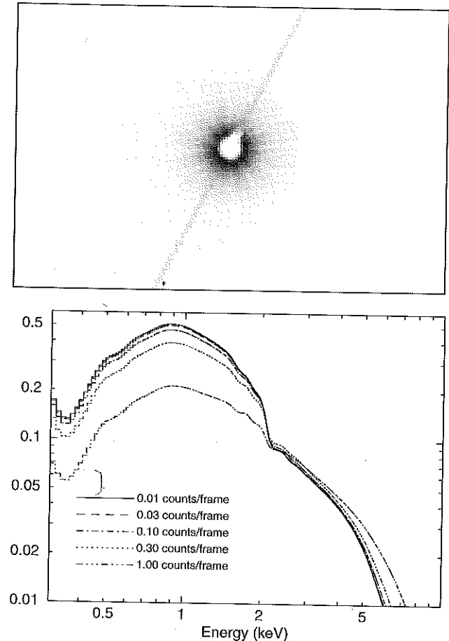
Fig. 4.5 [Top] Chandra ACIS observation of the bright source Hercules X-1. The hole in the center of the source is due to piled-up events which are rejected because of bad grades. Also visible are the streaks due to events detected while the detector is being read out and the shadows of the mirror support structure. [Bottom] Chandra ACIS simulated spectra showing the effect of increasing pileup. As the input count rate, and hence pileup, is increased the observed spectrum decreases at low energy while increasing at higher energies
