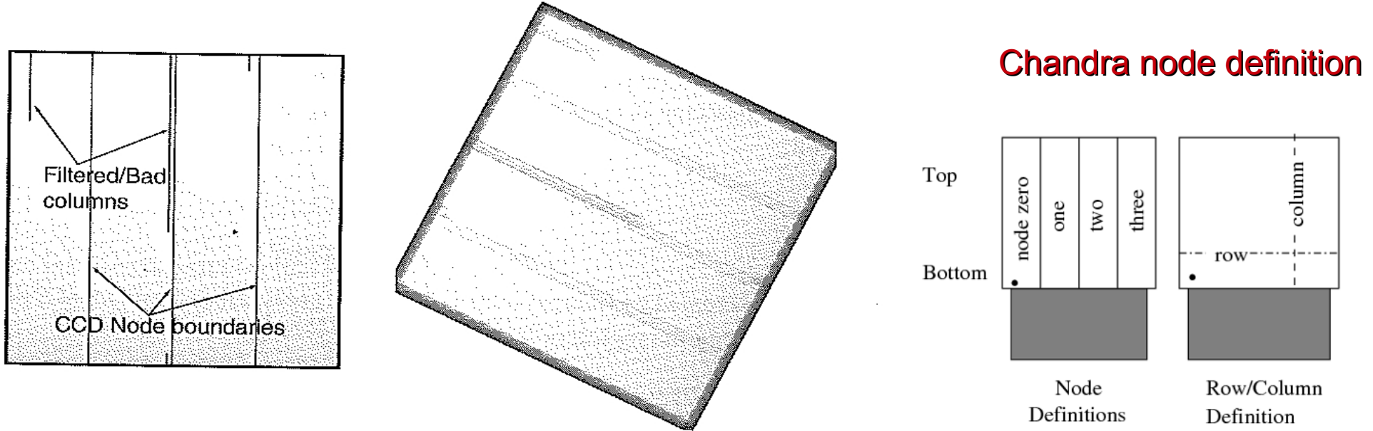
Fig. 4.10 [Left] Chandra ACIS instrumental effective area (exposure) map (at 1.5 keV) in detector coordinates, showing the node boundaries on the CCD and undesirable or bad columns that have been filtered. [Right] Same, after converting to sky coordinates and including the ACIS dither that smears out the bad columns
